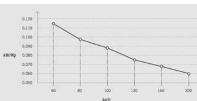
Figure 5: Reduction in power consumption for combed yarn by Marzoli's card model
